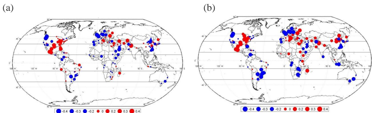
Fig. (6). Global distribution of daytime LST trends for the world's 233 largest cities (populations exceeding 2 million) during the 11-year period 2002-2012, based on LST data sets retrieved from (a) Terra -MODIS (176 cities) and (b) Aqua -MODIS (169 megacities) at 1^\circ \times 1^\circ horizontal intervals. Months with cloudiness exceeding 0.7 and cities with less than 6 years of data availability were not included.
