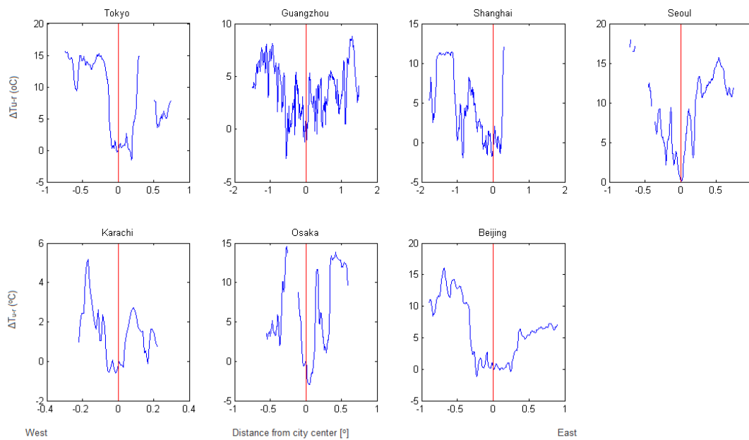
(a) Latitudinal distribution of 12-year mean during daytime
