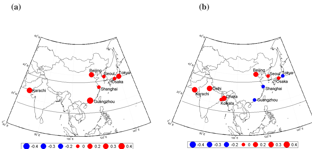
Fig. (8). Aqua -MODIS LST trends during daytime (a-left panel) and nighttime (b-right panel), for the June-August during 2003-2014, based on 1 km Aqua -MODIS. Note that blue/red color indicates negative/positive trends. Cities with incomplete data are Karachi (2002-2011), Dhaka (2002-2013), Delhi (2002-2008) and Kolkata (no daytime records).
