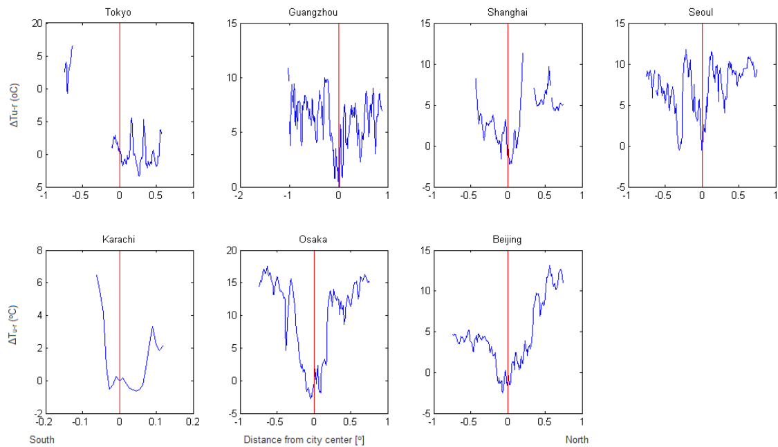
(a) Longitudinal distribution of 12-year mean during daytime
