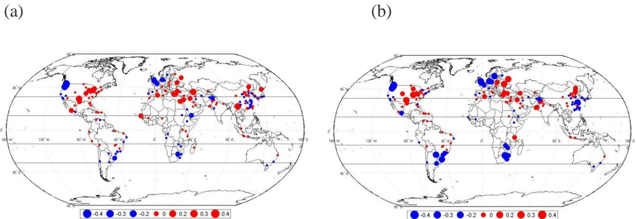
Fig.(7). As in Fig. (6) but for nighttime based on LST data sets of (a) Terra -MODIS (179 cities) and (b) Aqua -MODIS (172 megacities) at 1^\circ \times 1^\circ .
